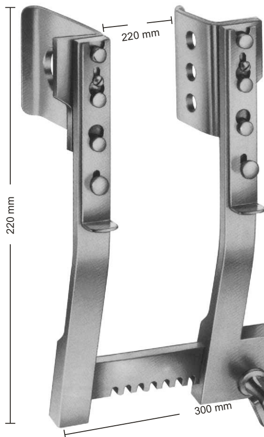
17-394 FINOCHIETTO-BURFORD with 2 pairs of blades
