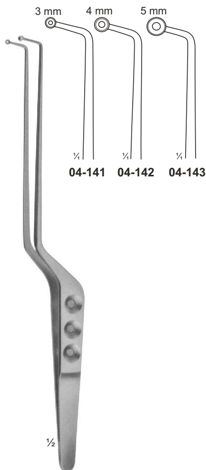
04-141 - 143 SAMII Jaws Spoon-Shaped 230 mm
