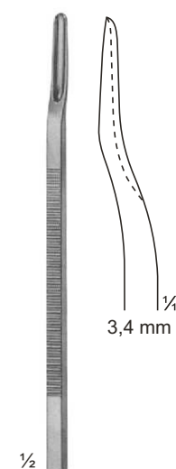
21-130 Scaphoid gouge, downwards curved 135 mm
